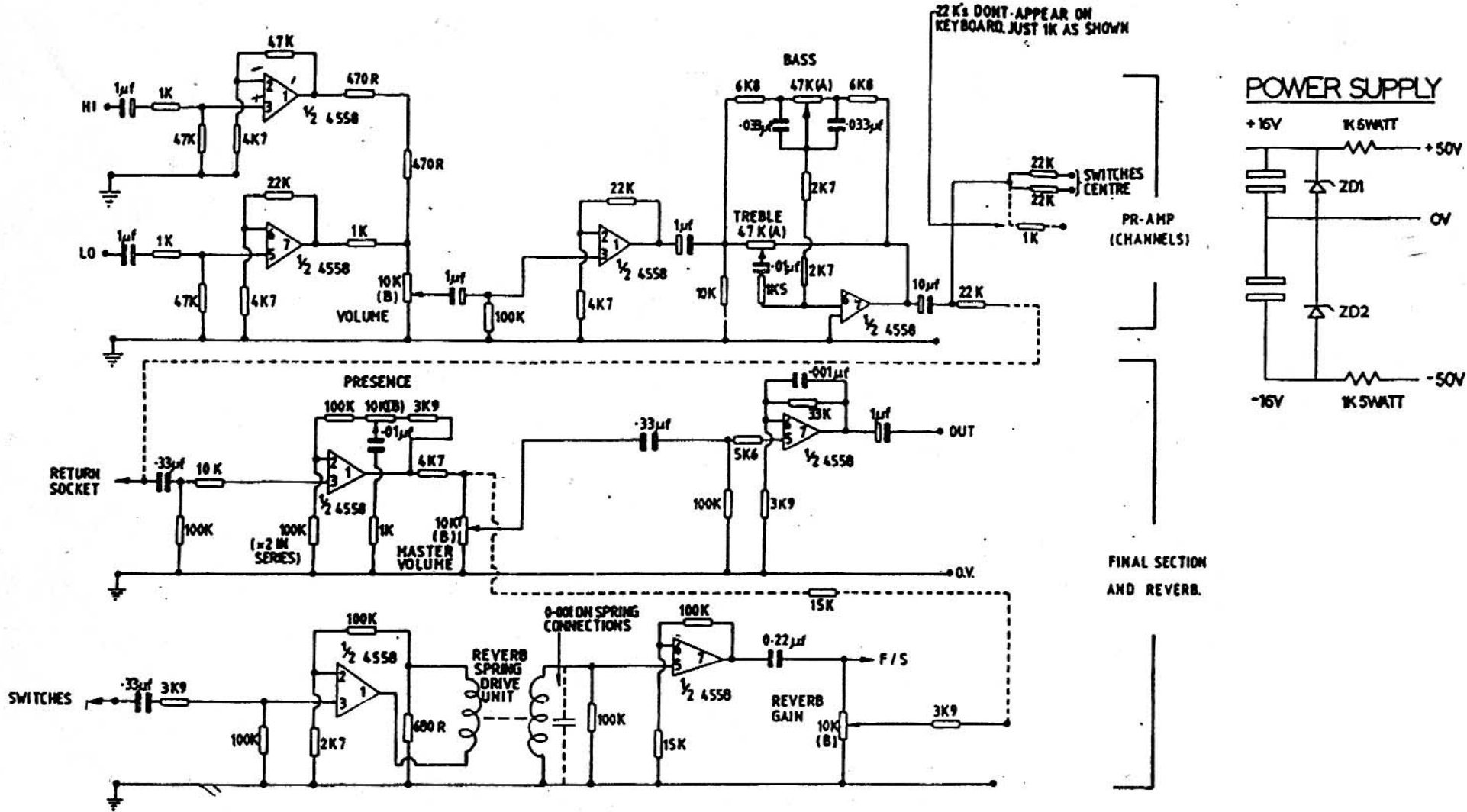
Vox Venue Keyboard 100 & PA120/PA200 Pre-Amp
